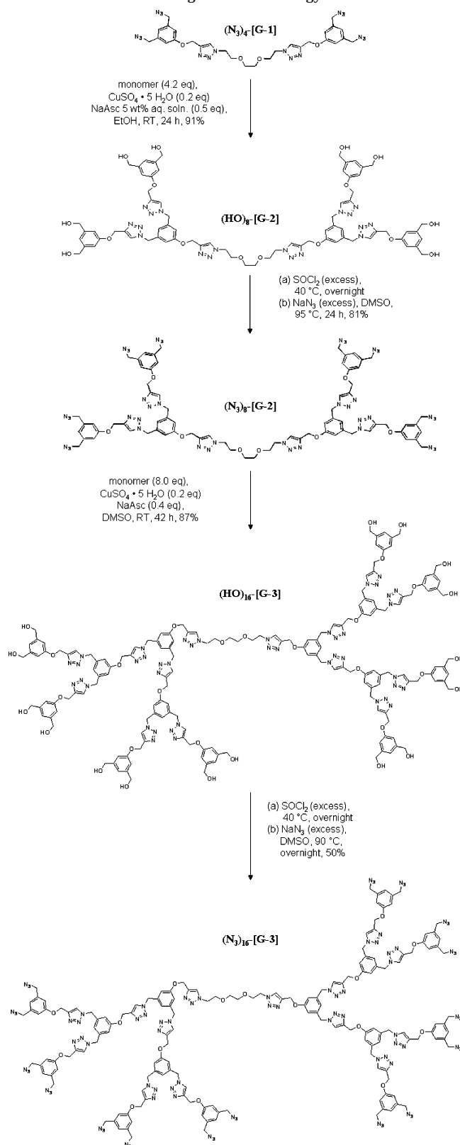
Scheme 3. Synthesis of Generation 2 and 3 Dendrimers by a Divergent Click Strategy
